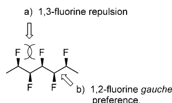
Figure 1. Multivincinal fluoroalkane conformation is governed by a) the avoidance of 1,3-fluorine repulsion and b) the 1,2-fluorine gauche effect.
